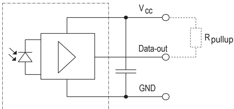
Figure 1. Block Diagram
